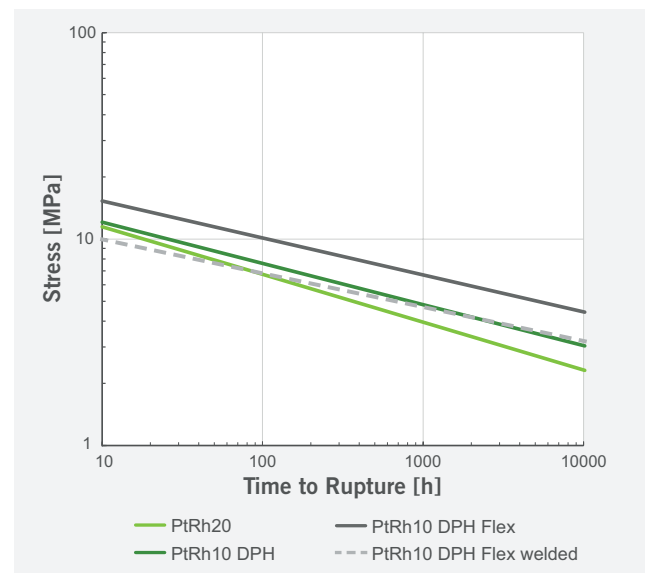
Rupture 1400°C
